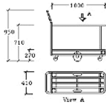
TS/055 - Double Deck Tubular Stock Trolley
