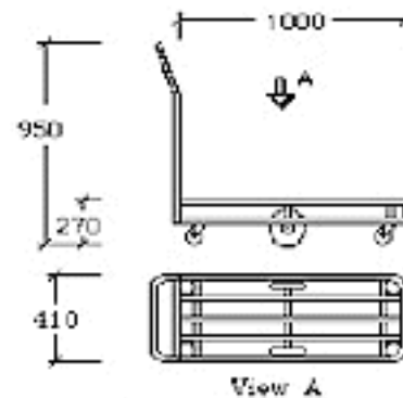
TS/005 - Single Deck Tubular Stock Trolley
