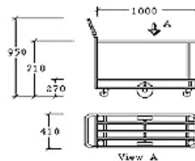
TS/015 Double Deck Tubular Stock Trolley
