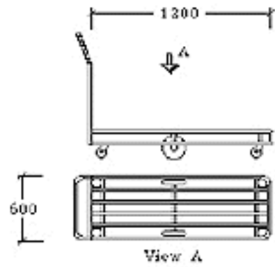
TS/045 Single Deck Tubular Stock Trolley
